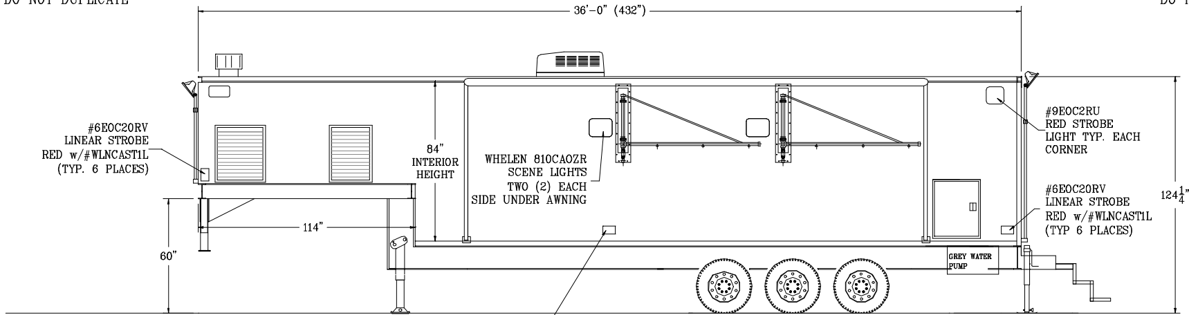
STREETSIDE ELEVATION
