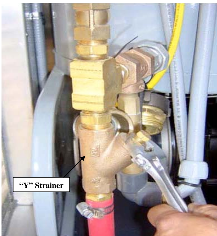
Fig. 2 Inlet Strainer
