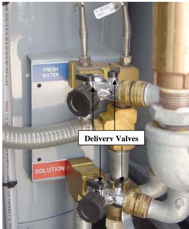
Fig. 5 Water Heater Delivery Valves
