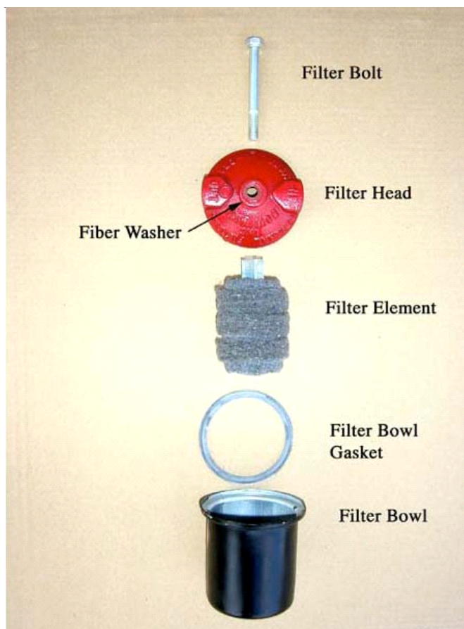
Fig. 10 Fuel Filter - Breakdown
