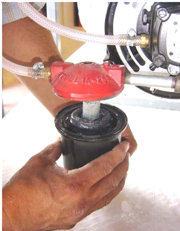
Fig. 9 Fuel Filter – Fiber Element
