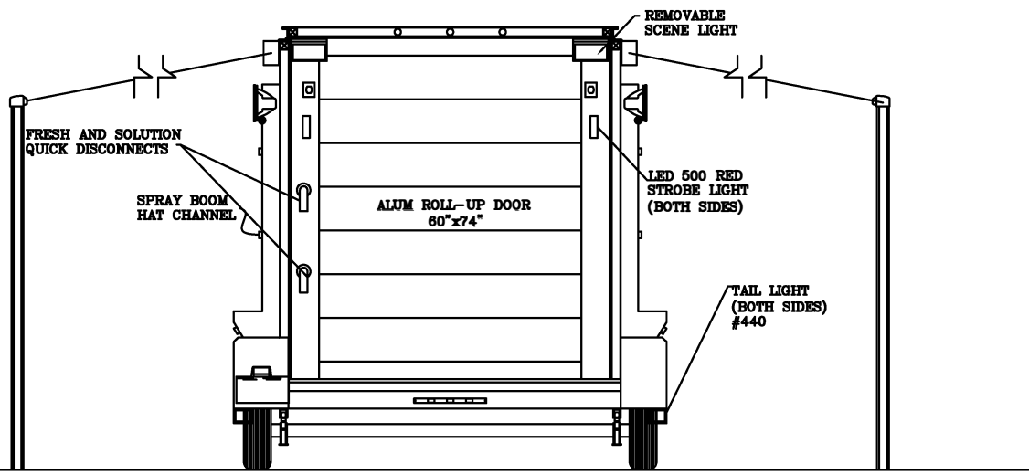
ELEVATION LAYOUT REAR SIDE
