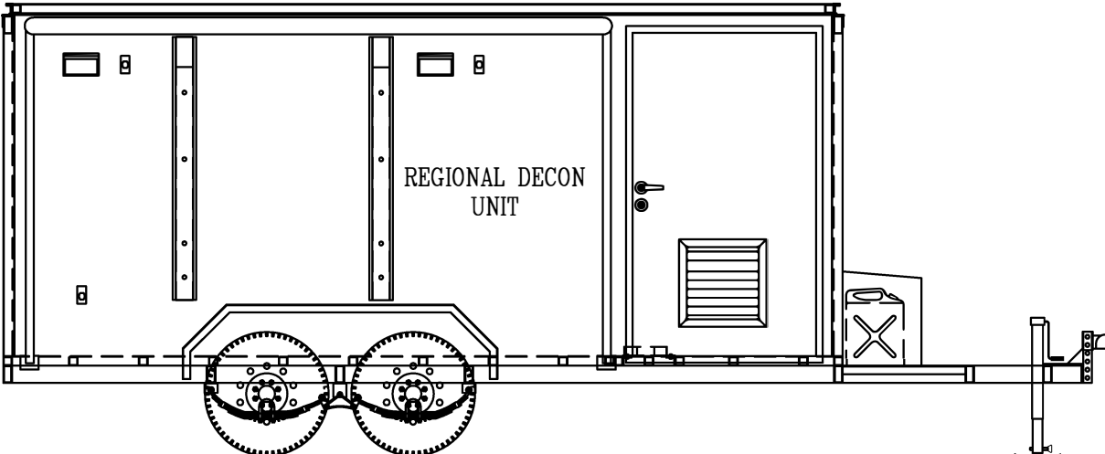
ELEVATION LAYOUT CURBSIDE
