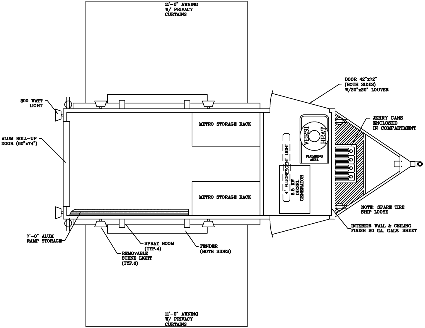
FLOOR PLAN LAYOUT
